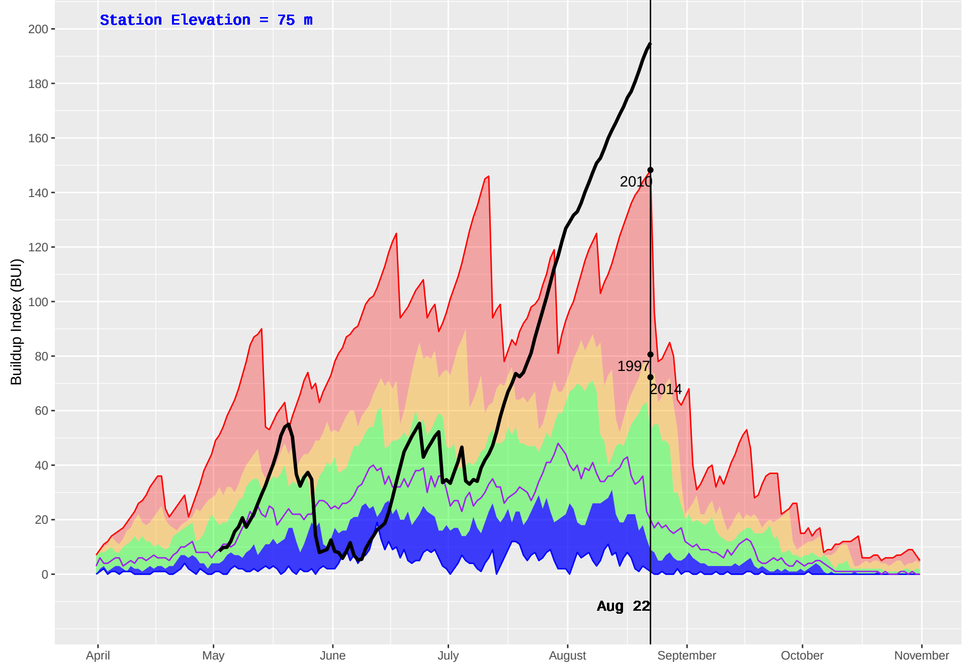
KITPARK (106) : Historical (1995–2016) and Current (2018) Daily Buildup Index (BUI)
